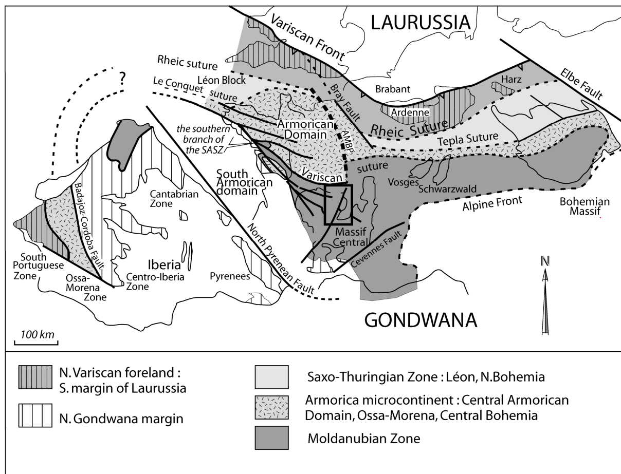
Figure 1 : Structural map of the Variscan domain in western Europe [after Faure, 2005]
