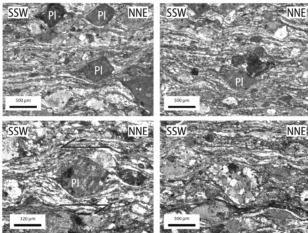
Figure 9 : Thin section pictures of the mylonites from the “Proto Sillon Houiller”.
