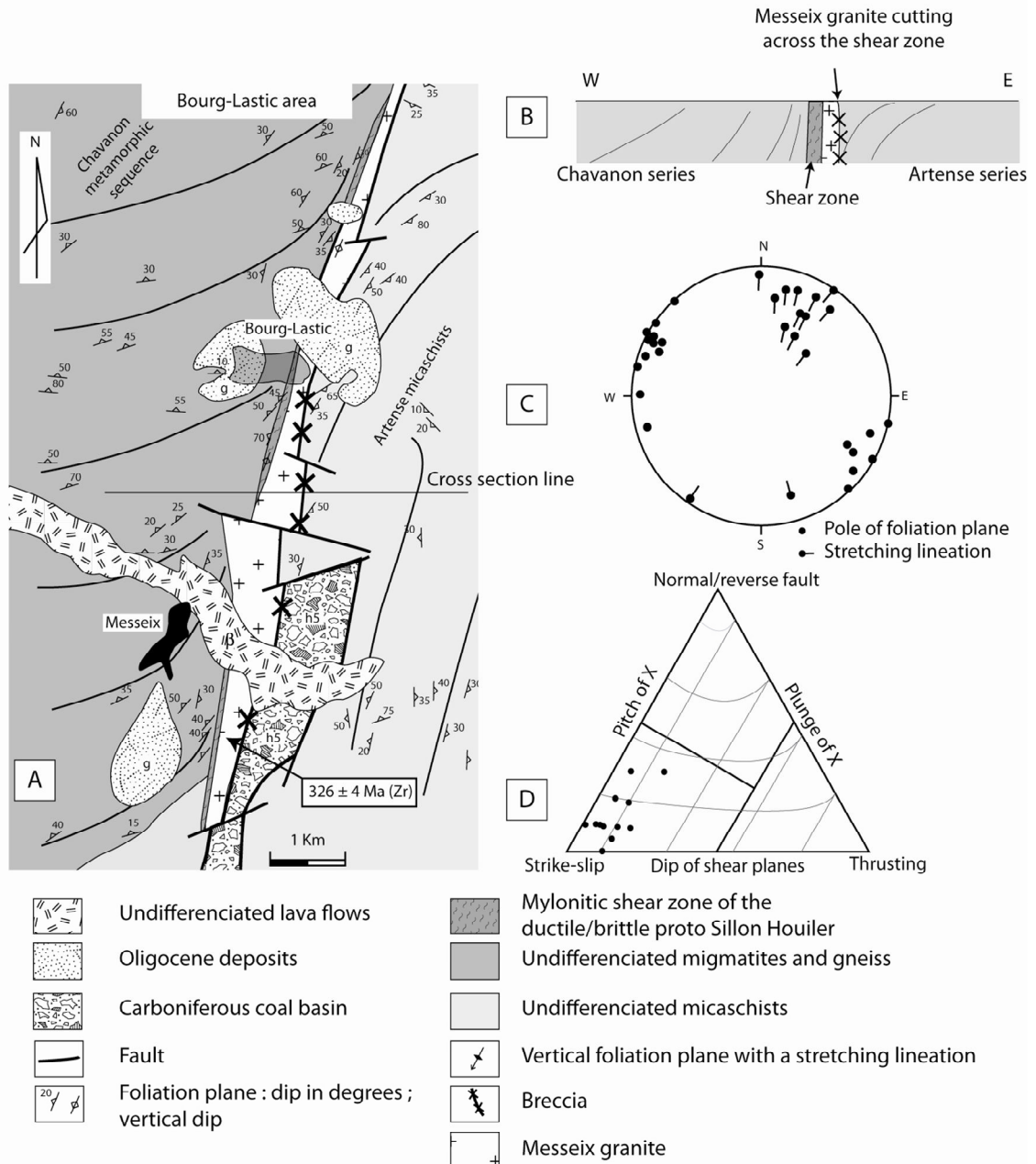
Figure 3 : a) Geological map of the Bourg-Lastic area showing the mylonitic shear zone of the proto-Sillon Houiller cross-cut by the Messeix granite, b) simplified cross-section of the area, c) Stereogram of structural data collected along the proto-Sillon Houiller, d) Projection of the structural data in Rickard's diagram [1983] proving a strike-slip offset of the fault.
