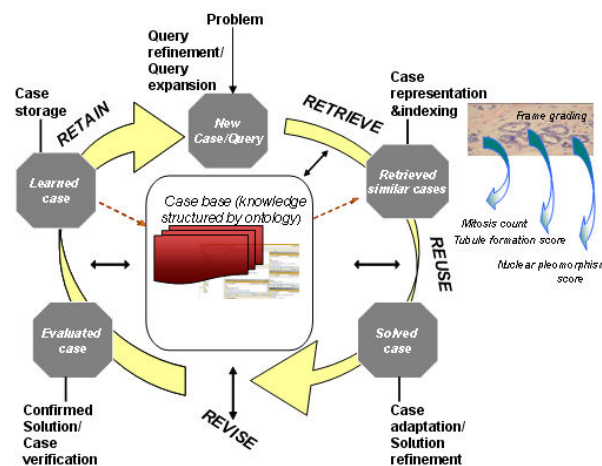
Figure 3.2. CBIR-CBR strategy
