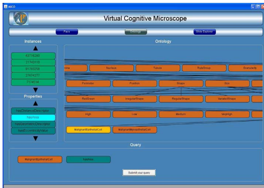
Figure 8.8. Ontology management
