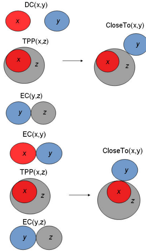
Figure 5.4. CloseTo relation
